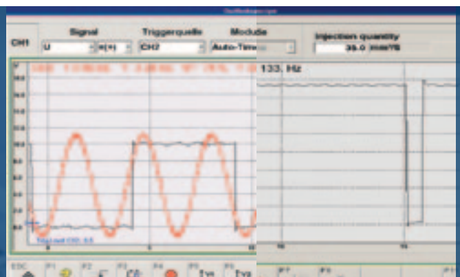
2-channel oscilloscope for optimum troubleshooting
